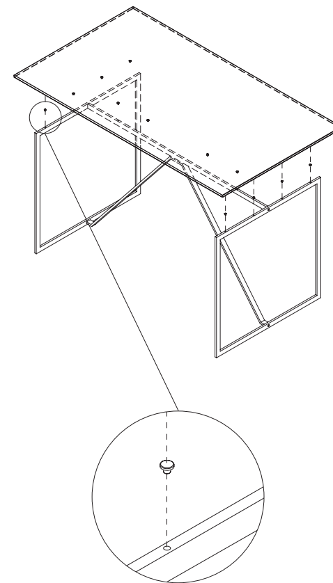
(g) Appoggi per piano in vetro Support for glass
